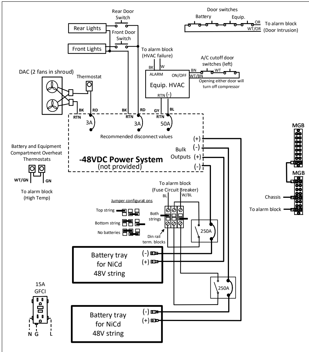
Figure 3 CUBE Electrical Diagram
