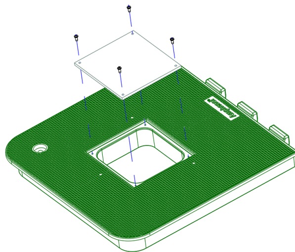
Figure 1 Vault Cover Installation
