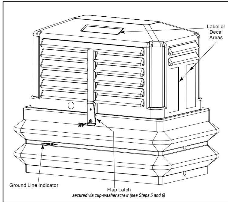
Figure 1. Typical CMPH Enclosure, Closed View
