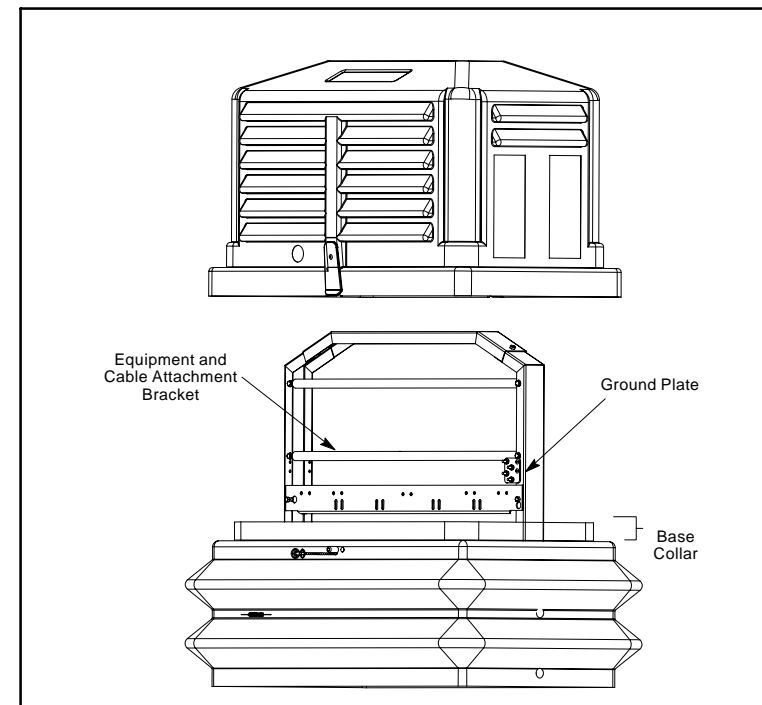
Figure 2. Typical CMPH Enclosure, Dome Lifted
