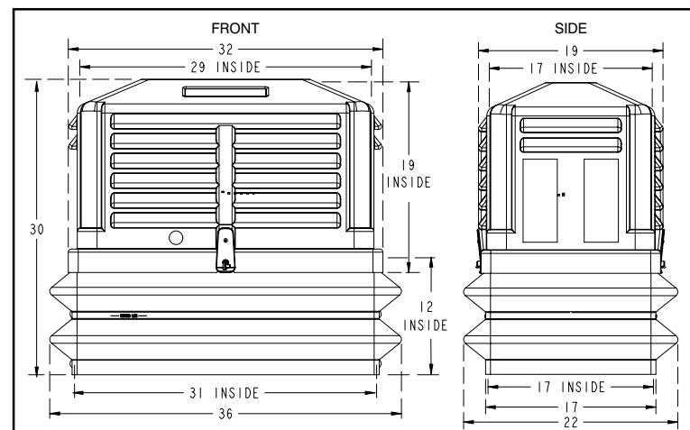
Figure 3. Front and Side Views of CMPH-5500
