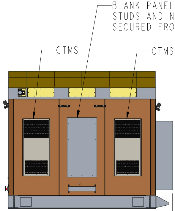
WIC LEFT SIDE VIEW
