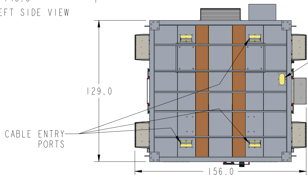
WIC BOTTOM VIEW
