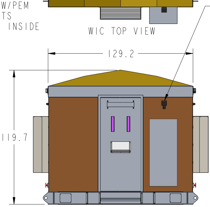
WIC FRONT VIEW
