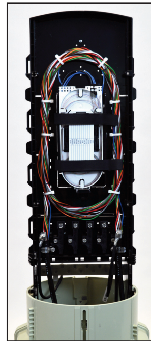
BDO205-EGT12/CL Backboard Views with Customer Installed Fiber (Left - Drop Side, Right - Feed Side)
