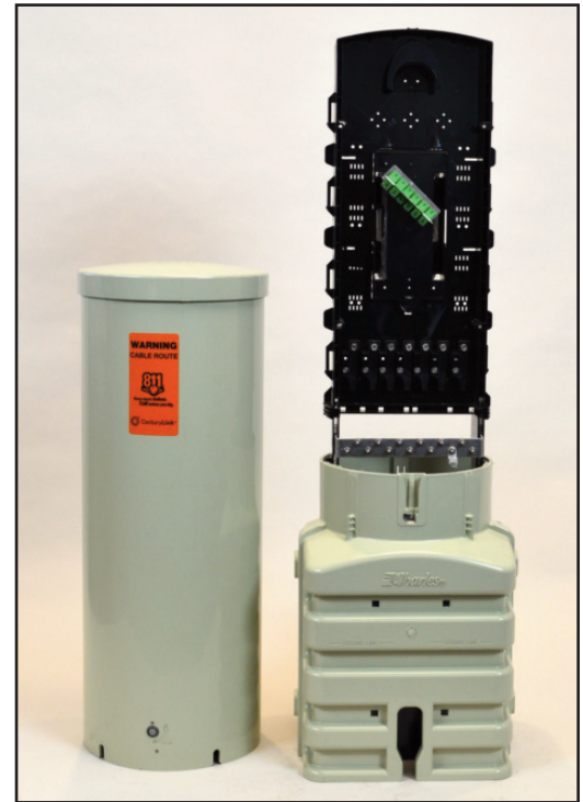
BDO205-EGT12/CL Pedestal (Drop Side)
