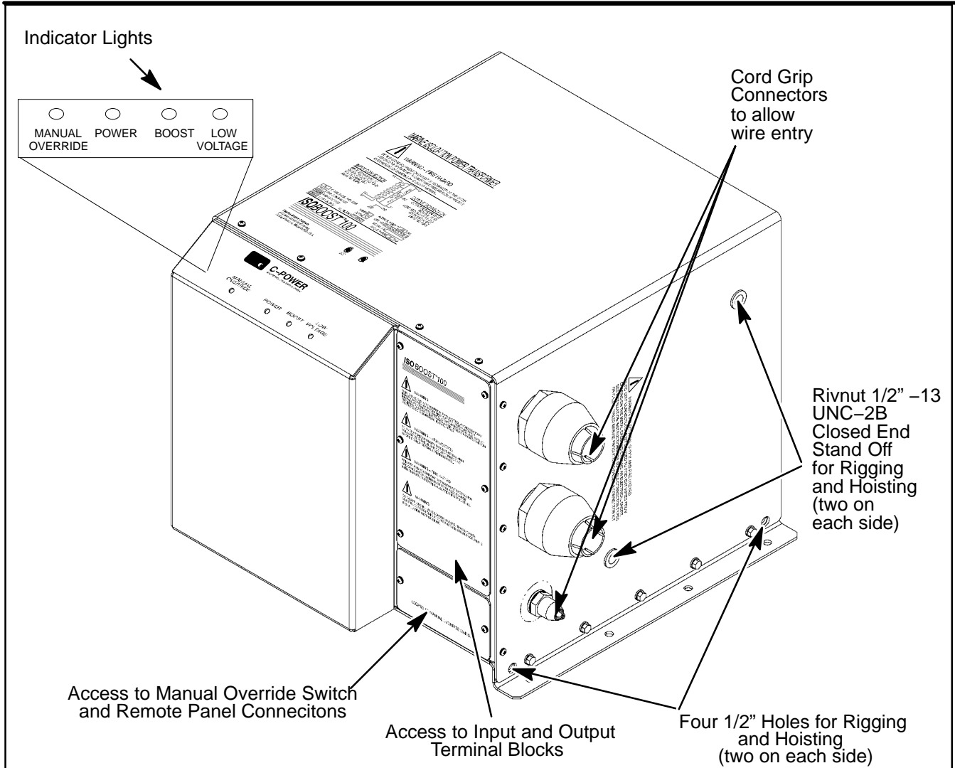
Figure 4. IsoBoost 100 Access Openings and Indicators
