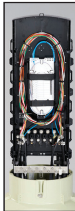
Fiber and Copper Co-Located Splices (for 10" and 14" diameter pedestals only)
