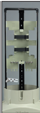
Fiber-Only Drop and Branch Splices (for 6", 8", 10" and 12" diameter pedestals only)
