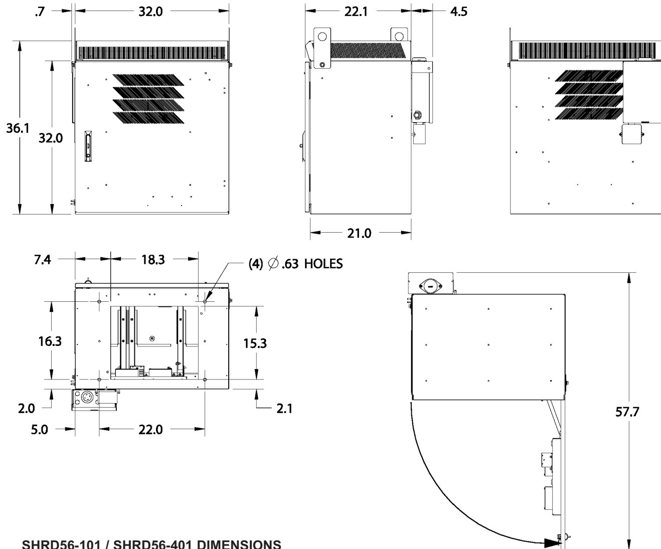
SHRD56-101 / SHRD56-401 DIMENSIONS
